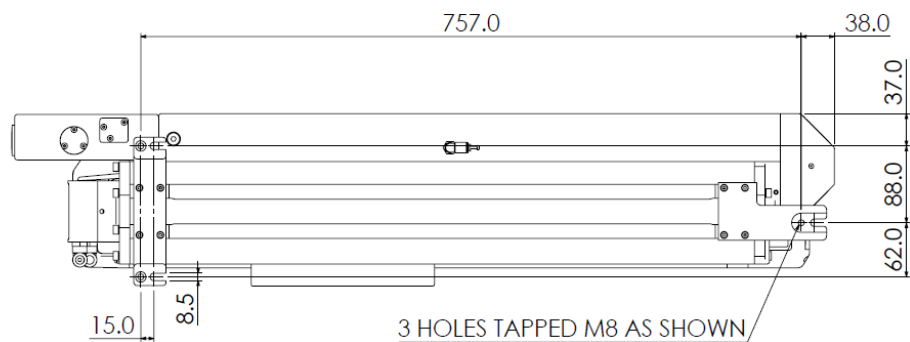
SR 15e – with shutter and diode assembly - optional
