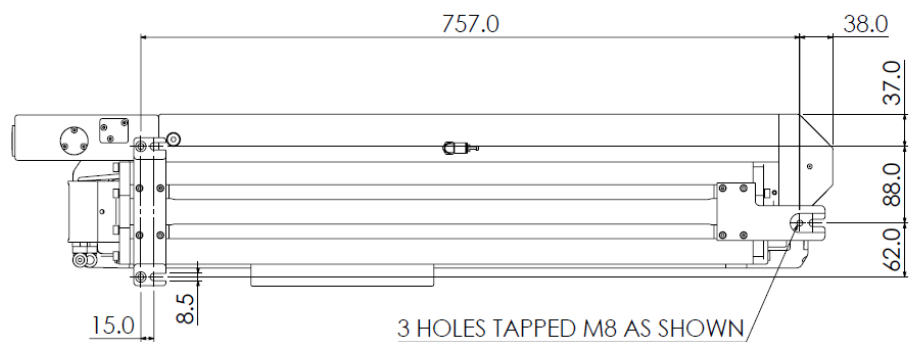
SR 15x – with shutter and diode assembly - optional
