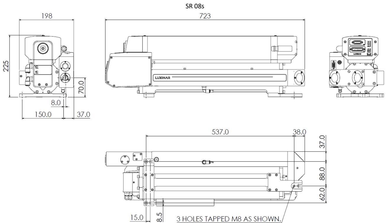
SR 08s – with shutter and diode assembly - optional
