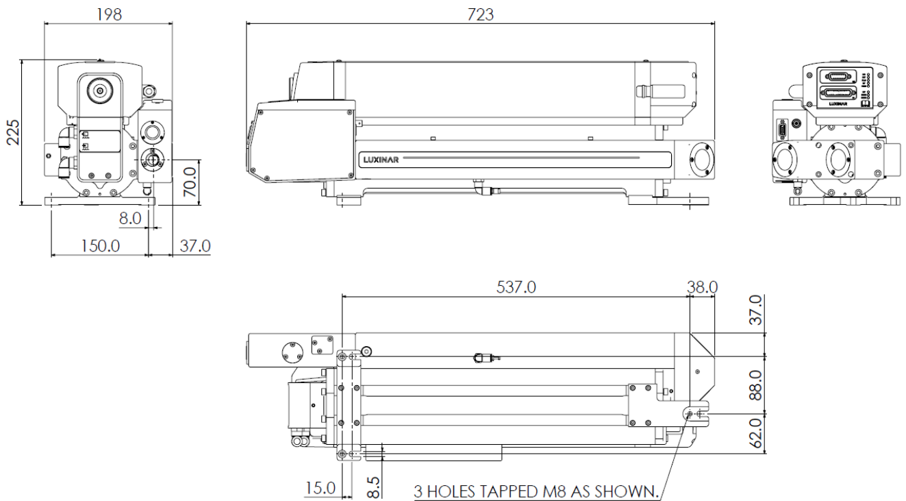
SR 08s – with shutter and diode assembly - optional
