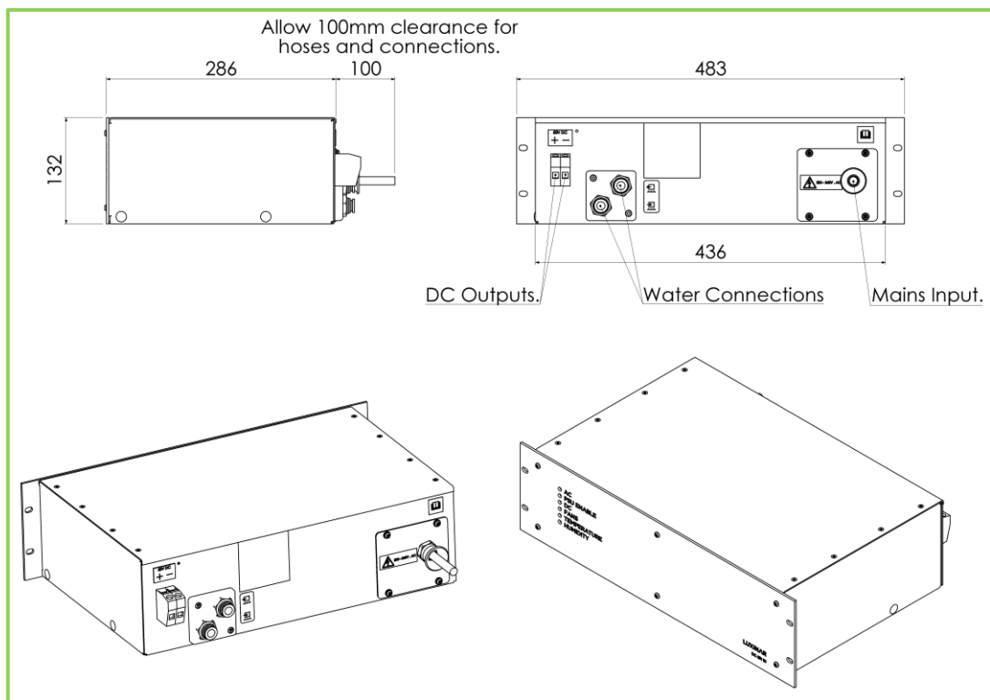
DC power supply – water cooled - 50V - optional
