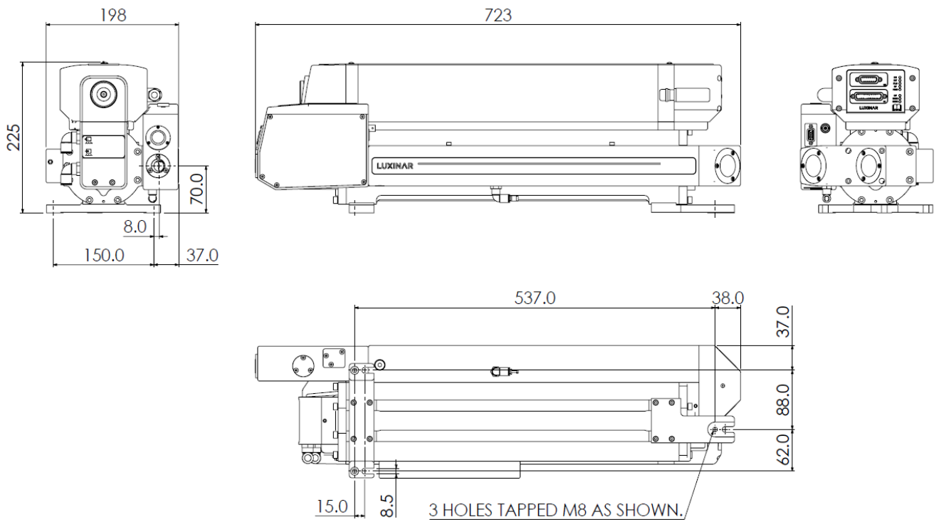
SR 10i – with shutter and diode assembly - optional
