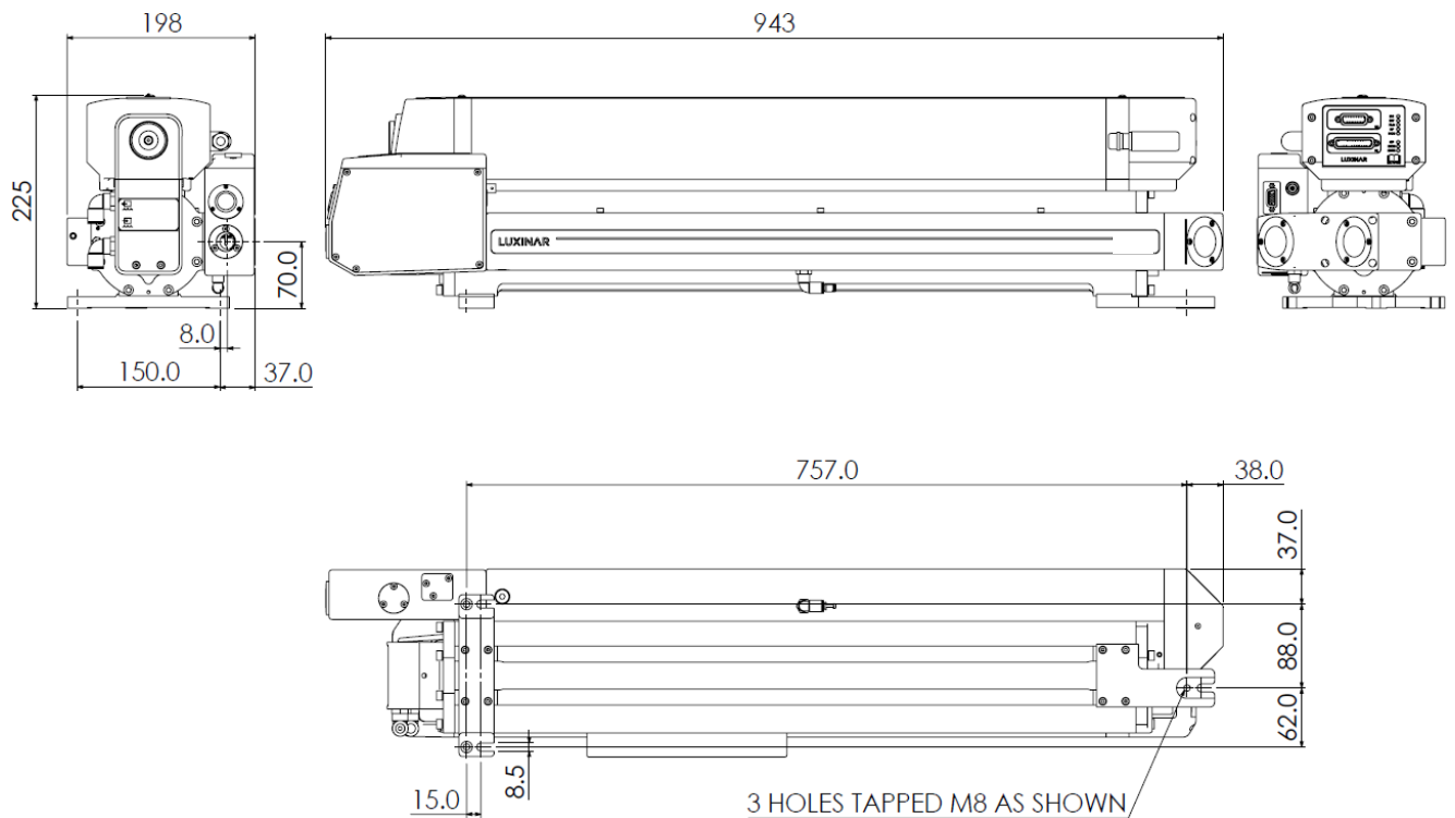
SR 15i – with shutter and diode assembly - optional
