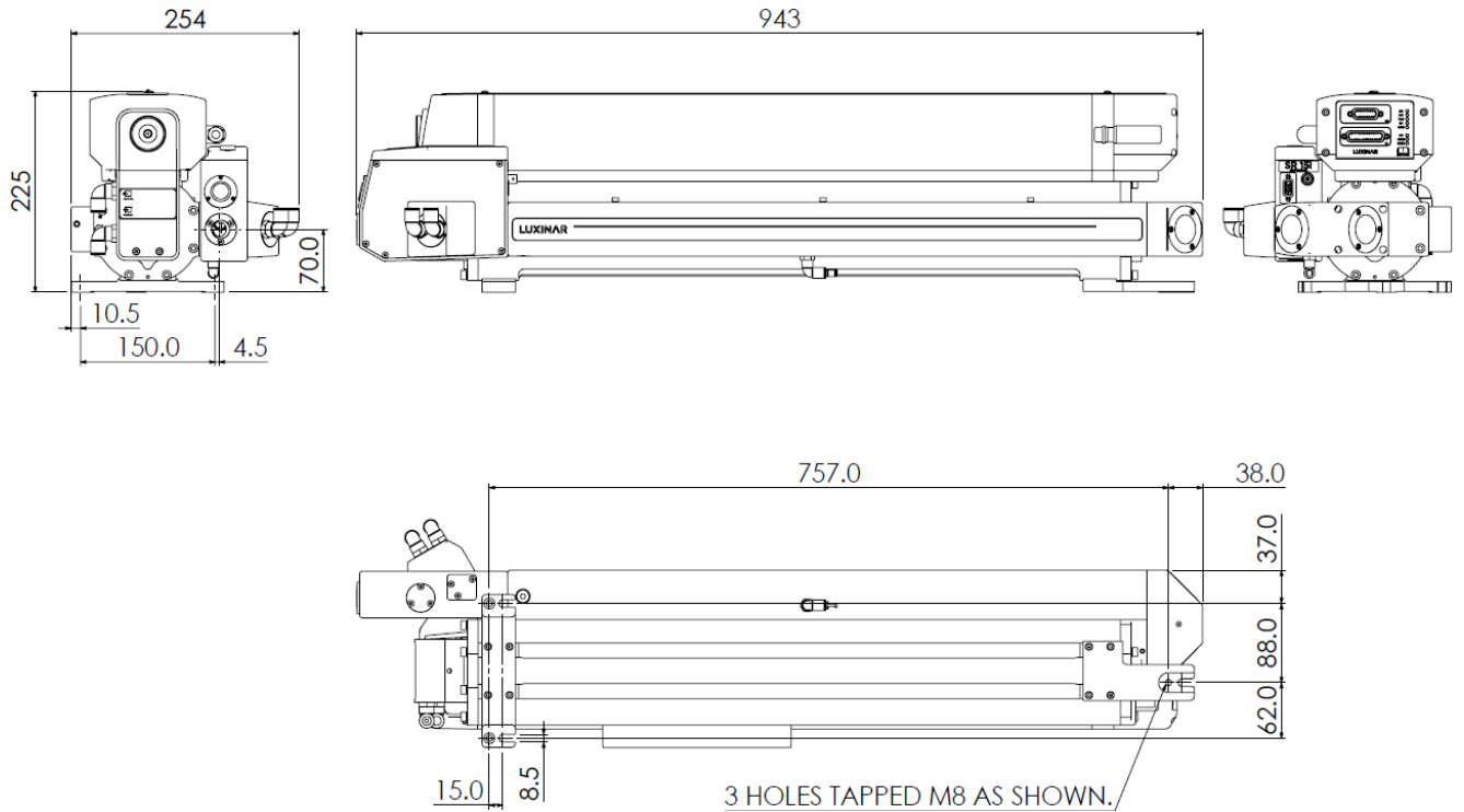
SR 15i – with shutter, diode and power feedback assembly – optional
