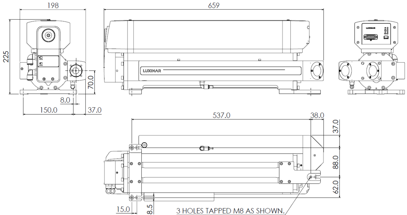
SR 10i
